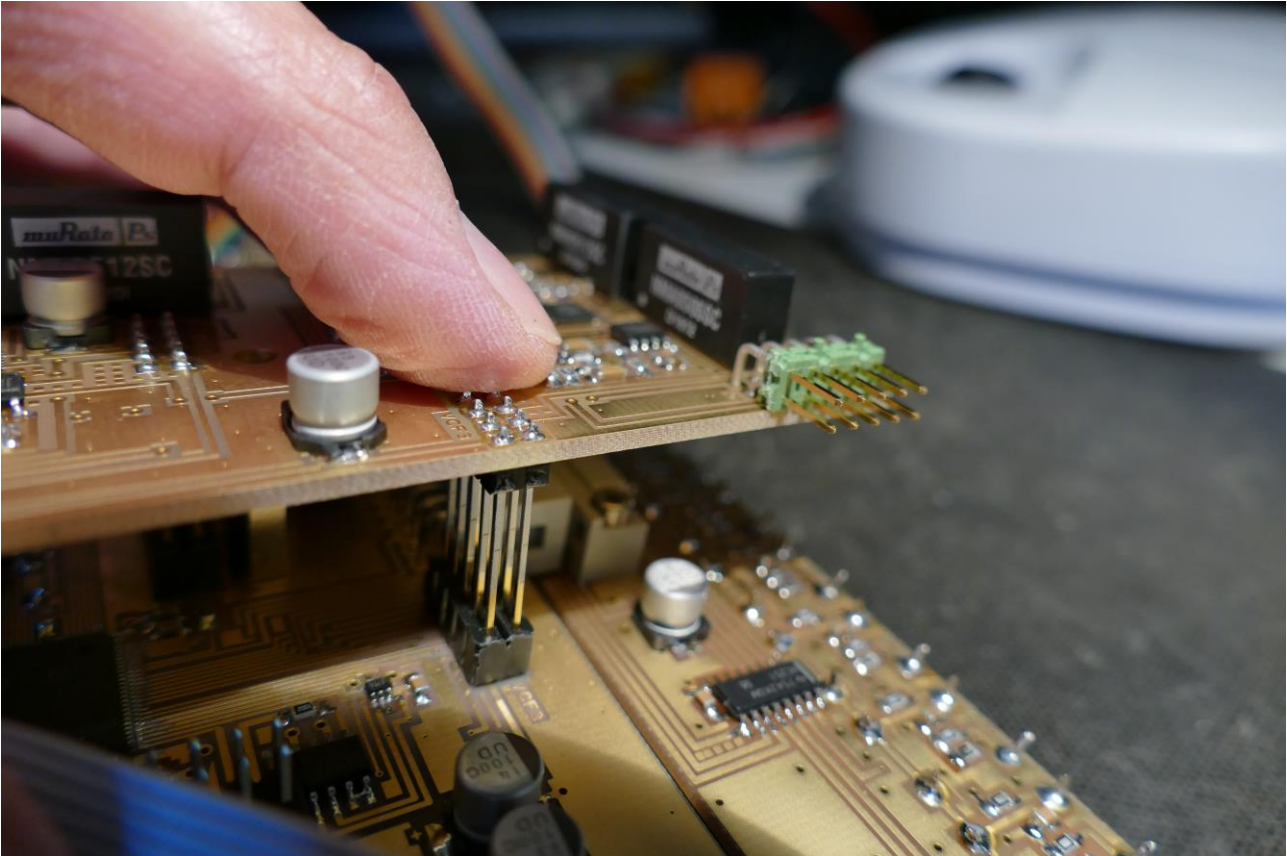
After making sure, that the connectors fits each other perfectly, press the analog board into these.
